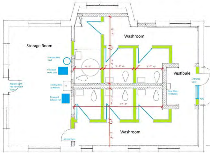
Creche Washroom SK-2 Proposed Layout
